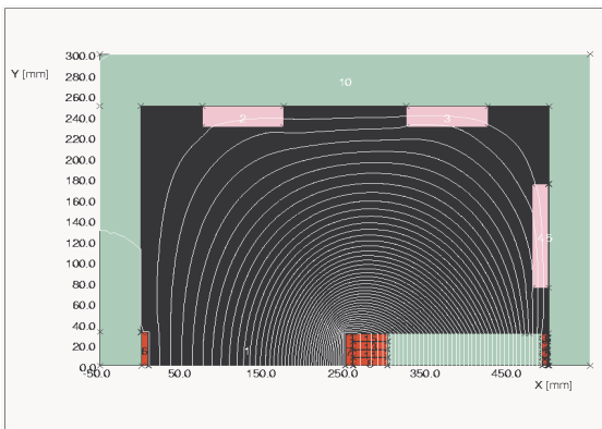
Fig2. Cross-section field distribution of CSRm Ex. septum
