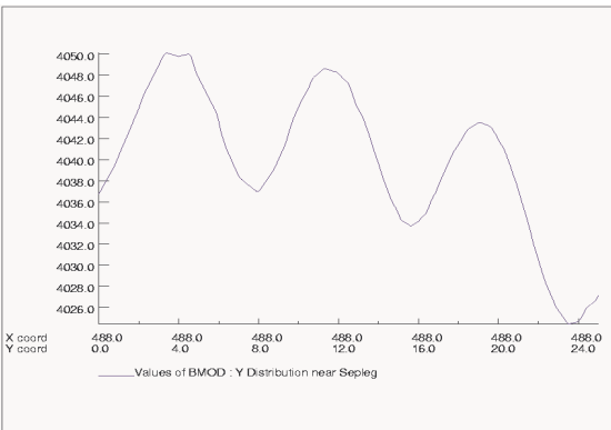
Fig5. Field distribution of CSRm Ex. near septum leg along Y-direction
