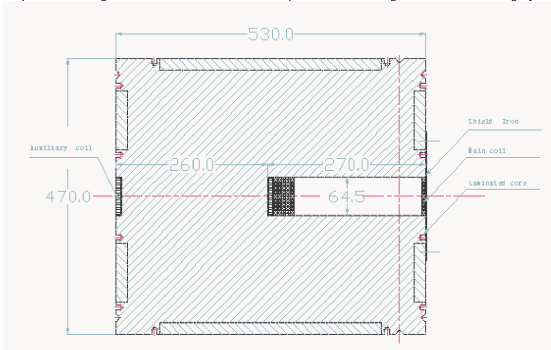
Fig 1. Cross section of the CSRm Ex. magnetic septum
