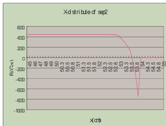
Fig3. 2-D field distribution of CSRm Ex. Septum along X-direction
