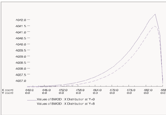
Fig4. Field distribution of CSRm Ex. in aperture along X-direction
