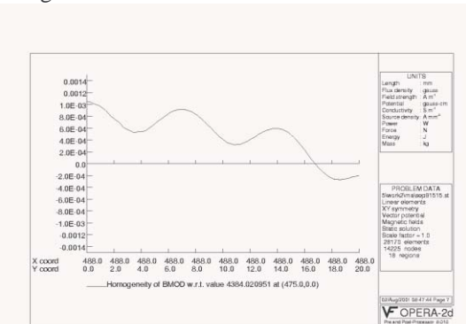
Fig6. Optimized field distribution near septum leg along Y-direction
